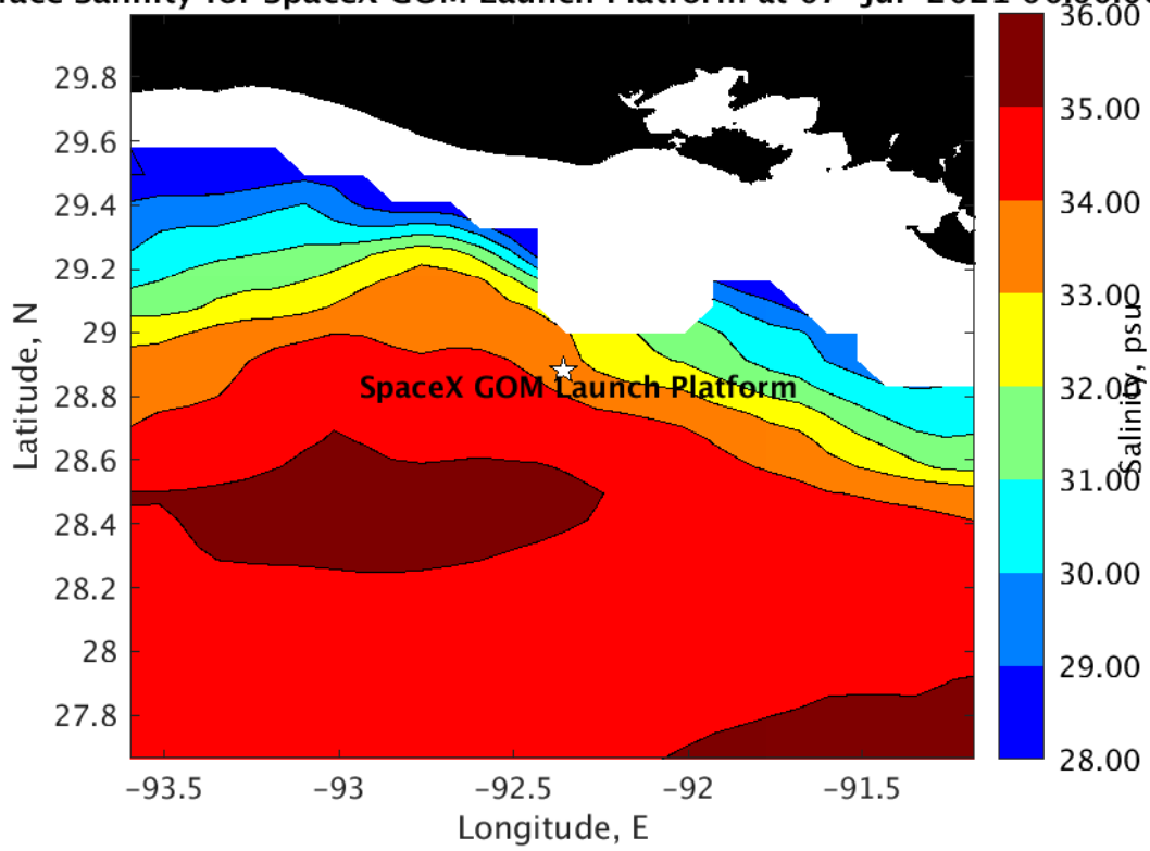
Surface Salinity for SpaceX GOM Launch Platform at 07-Jul-2021 00:00:00
